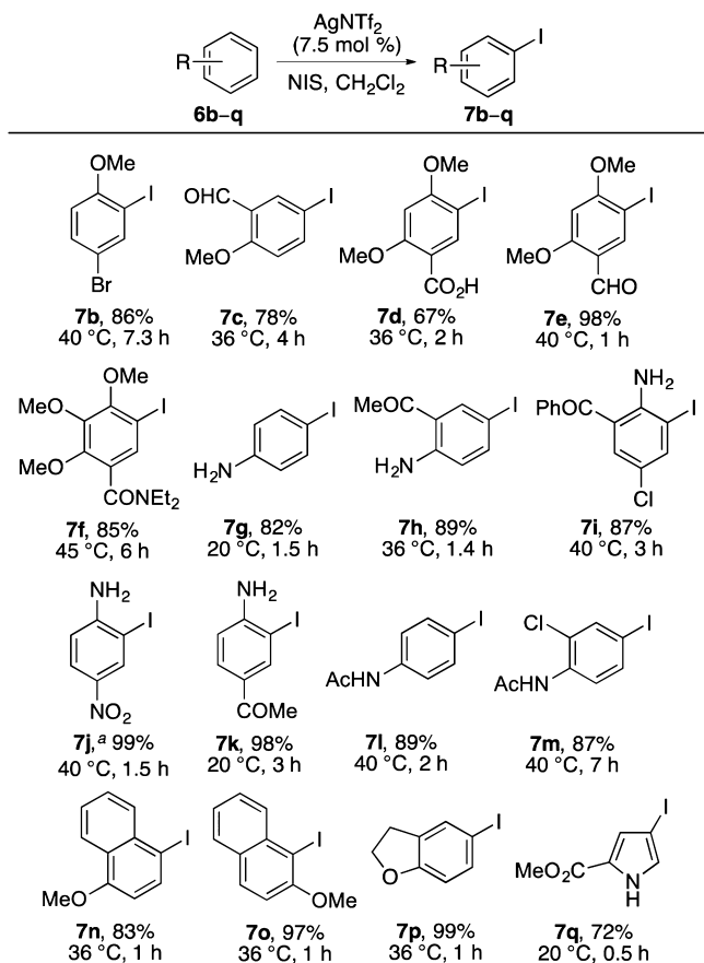
Scheme 2. Scope of Silver(I) Triflimide Catalyzed Iodination
