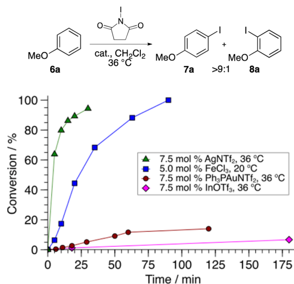
Figure 2. Iodination of anisole (6a) with various Lewis acids.
