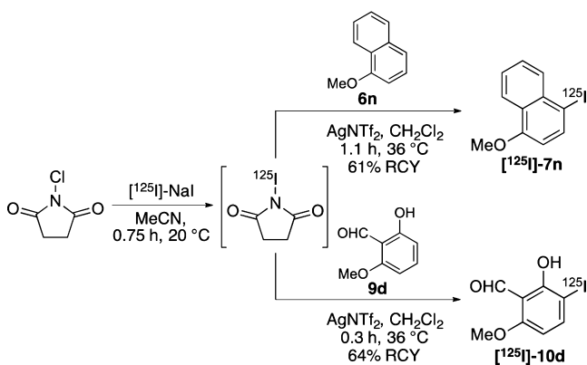
Scheme 5. One-Pot Radioiodination of 6n and 9d
