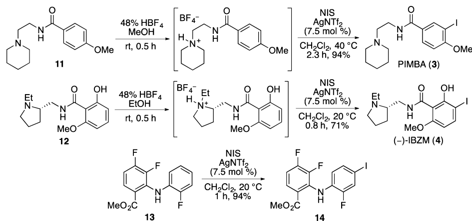
Scheme 5. One-Pot Radioiodination of 6n and 9d
