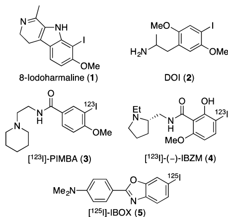
Figure 1. Structures of aryl iodide containing inhibitors and SPECT imaging agents.
