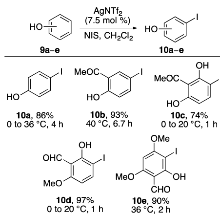
Scheme 3. Silver(I) Triflimide Catalyzed Iodination of Phenols
